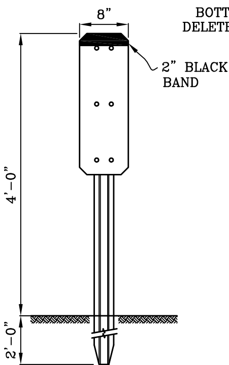
CULVERT MARKER
