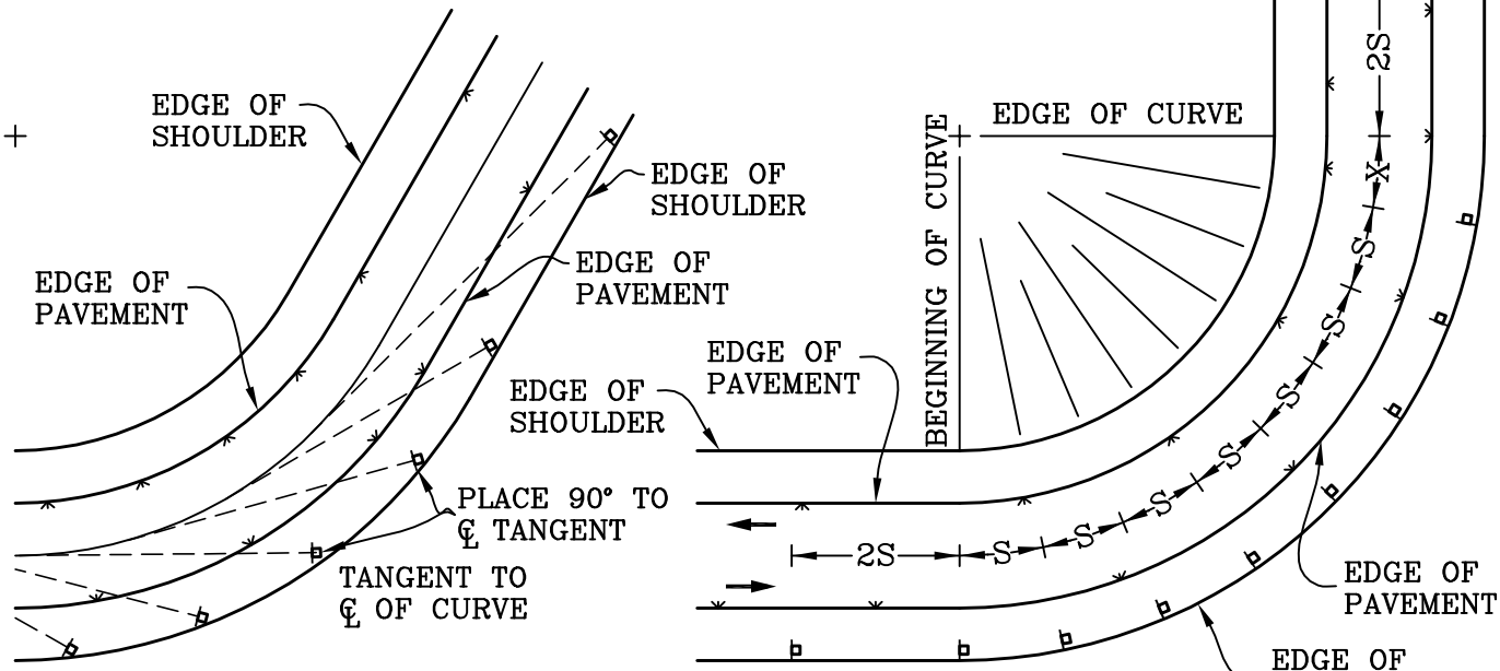
CURVE PLACEMENT DETAIL
